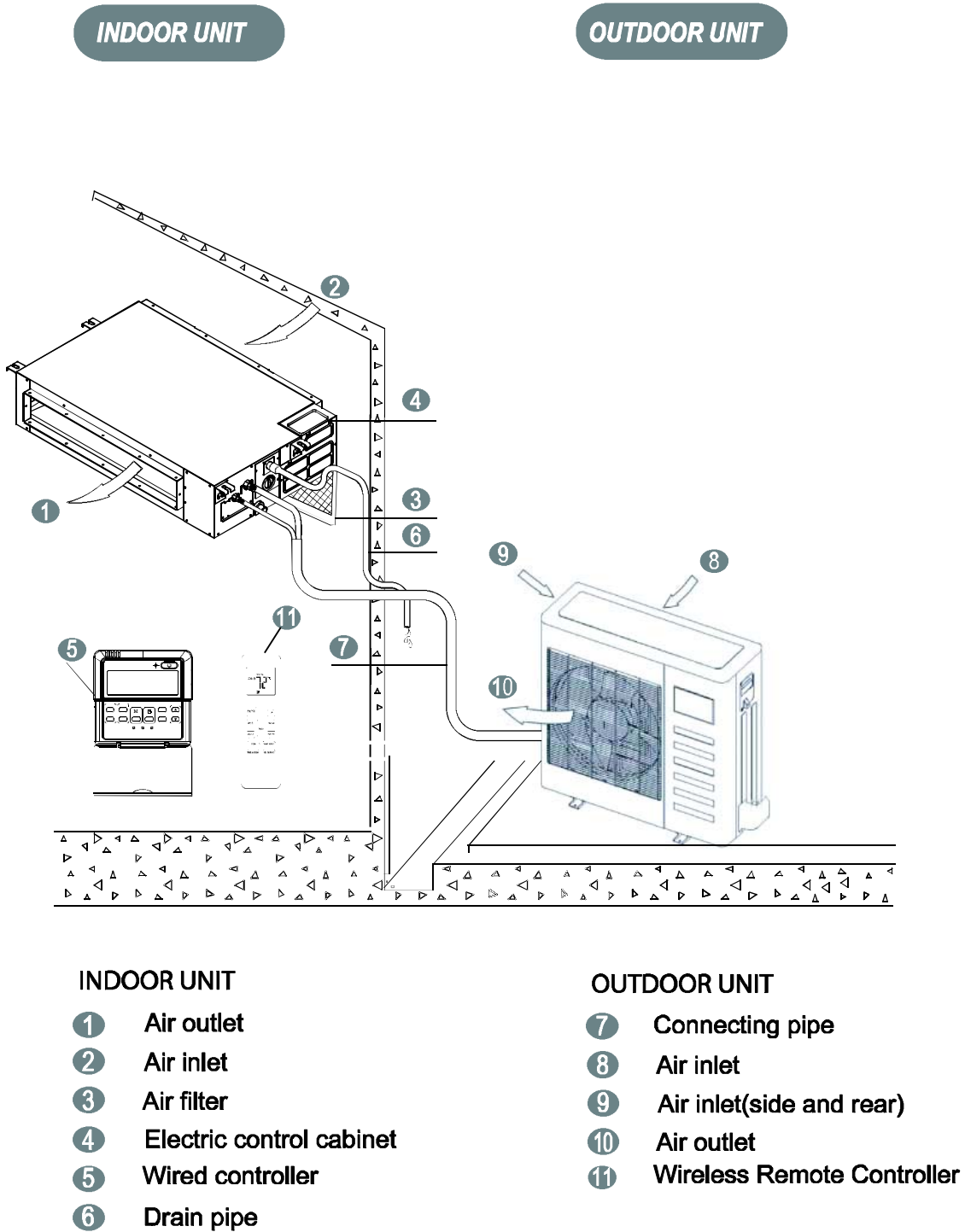
Fig. 1 - Indoor/Outdoor Unit
